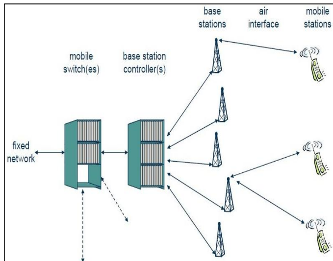
Fig. 1. Overview of microwave backhaul link to the GSM network
