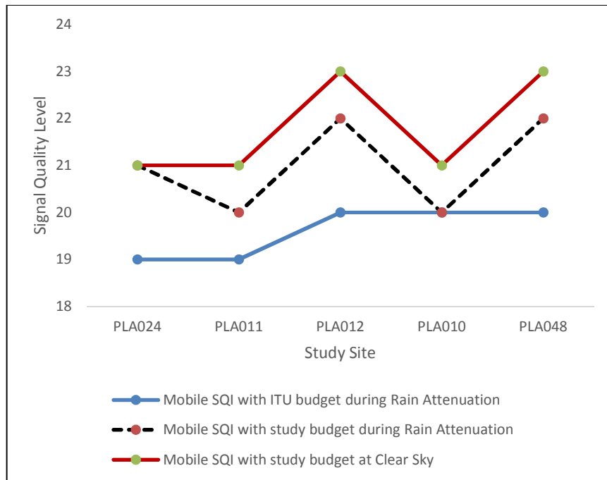
Fig. 5. 2G mobile SQL based on ITU-R budget compare to 2G mobile SQL based on study budget for Jos lowland cluster
