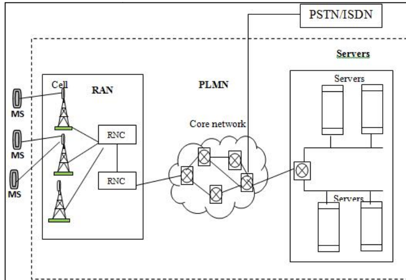
Fig. 3. 3G mobile network architecture
