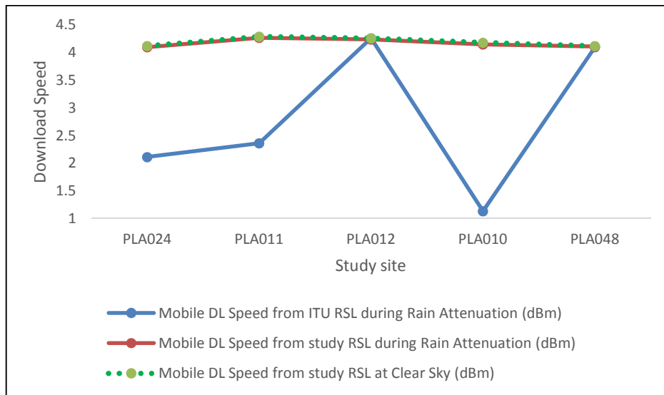
Fig. 4. 3G download speed based on ITU-R RSL compare to 3G download speed based on study RSL for Jos lowland cluster
