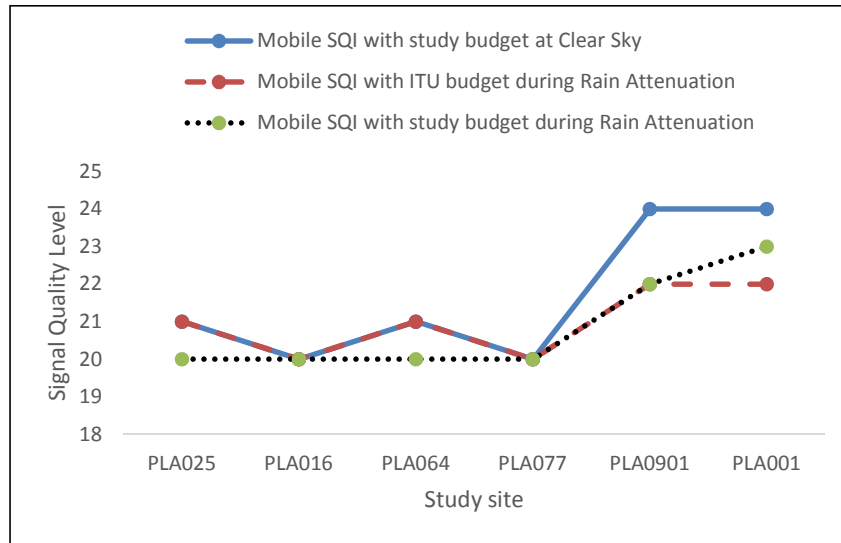
Fig. 7. 2G mobile SQL based on ITU-R budget compare to 2G mobile SQL based on study budget for Jos highland cluster
