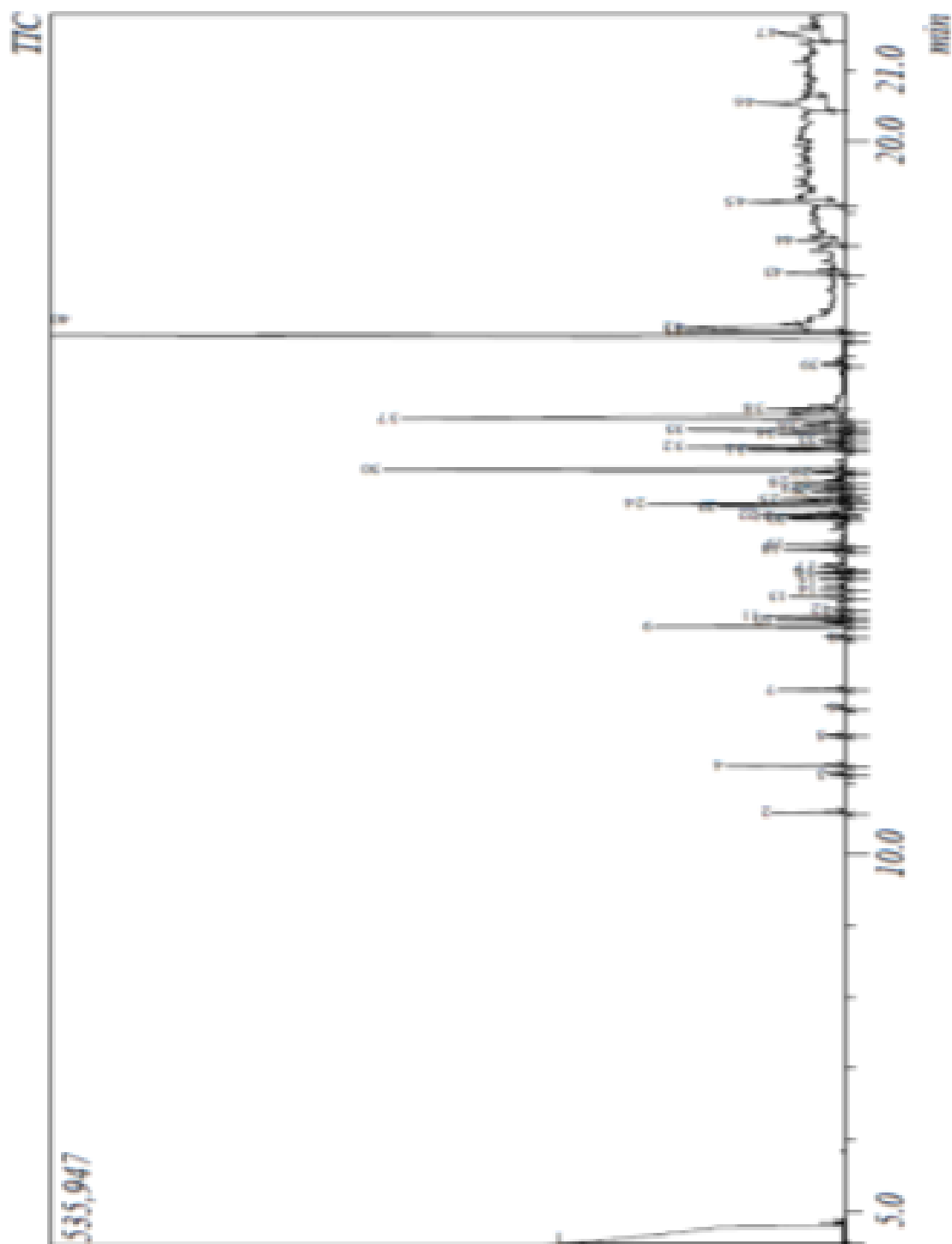
Fig. 1. GC-MS spectrum analysis of CDE of E. chlorantha stem bark
