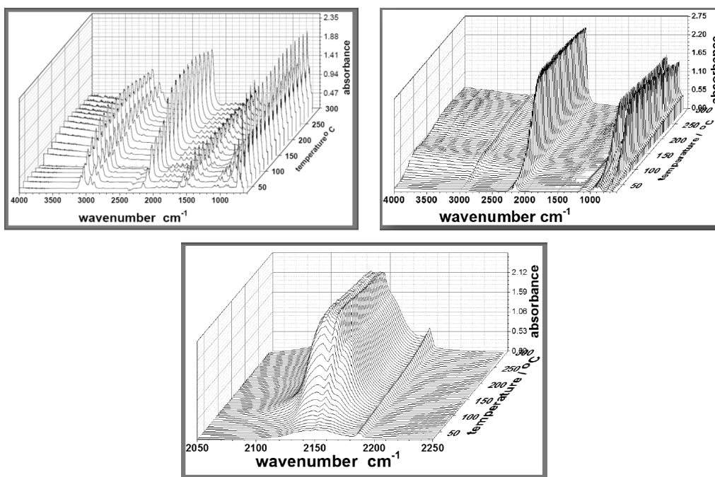
Fig. 4. The infrared spectra of CPS pure (right) and 20% CPS solution in toluene (left) recorded during heating the solution in steps of 5°C up to 270°C. Peaks between 2050 and 2250 cm -1 (bottom) which increases strongly for both types of CPS samples
