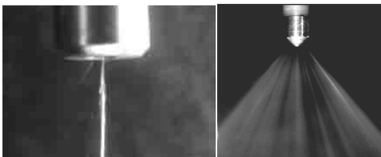
Fig. 2. Photographs of the ejecting aerosoles from the nozzle of high pressure injector under two different conditions
