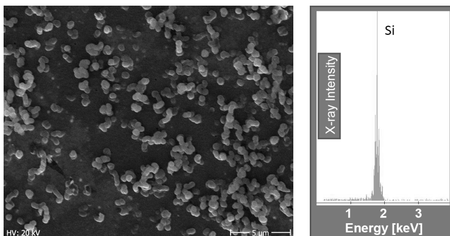
Fig. 6. (a) SEM image of a Si particles of deposited on a carbon glass plate from 20% CPS solution and annealed at 700°C for 20 min, the particle size corresponds to the size obtained by thermal decomposition, (b) The related EDXA curve
