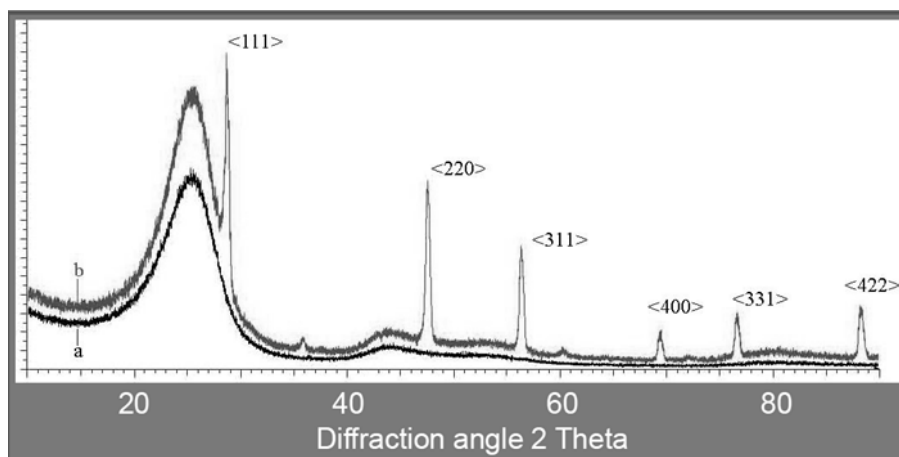
Fig. 9. The glancing incident x-ray diffraction patterns of silicon film deposited on carbon glass fiber from pure CPS and annealed at 950°C for 10 minutes. Curve with indices - polycrystalline diamond cubic structure Si
