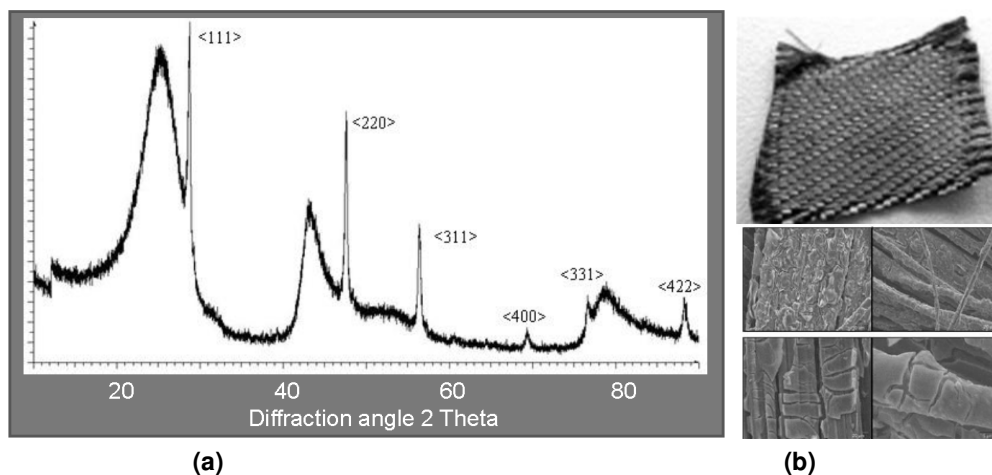
Fig. 7. (a) The glancing incident X-ray diffraction pattern of silicon film deposited from 20% CPS in toluene solution and annealed at 700°C. (b) Micrograph and SEM images of the samples
