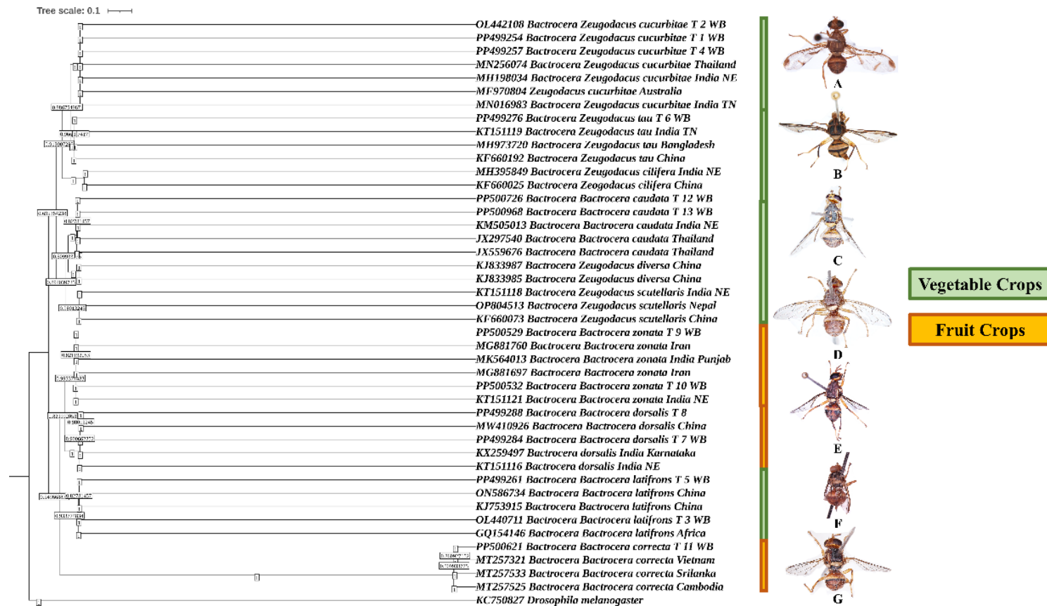
Fig. 4. The Bayesian (BA) Tree of 43 tephritid sequences with posterior probabilities from Bayesian analysis. Drosophilidae ( Drosophila melanogaster ) has been used as an outgroup. The different species are shown in this figure namely- (A) Bactrocera (Zeugodacus) cucurbitae (Coquillett, 1899), (B) Bactrocera (Zeugodacus) tau (Walker, 1849), (C) Bactrocera (Zeugodacus) caudata (Fabricius, 1805), (D) Bactrocera (Bactrocera) zonata (Saunders, 1842), (E) Bactrocera (Bactrocera) dorsalis (Hendel, 1912), (F) Bactrocera (Bactrocera) latifrons (Hendel, 1915), and (G) Bactrocera (Bactrocera) correcta (Bezzi, 1916)
